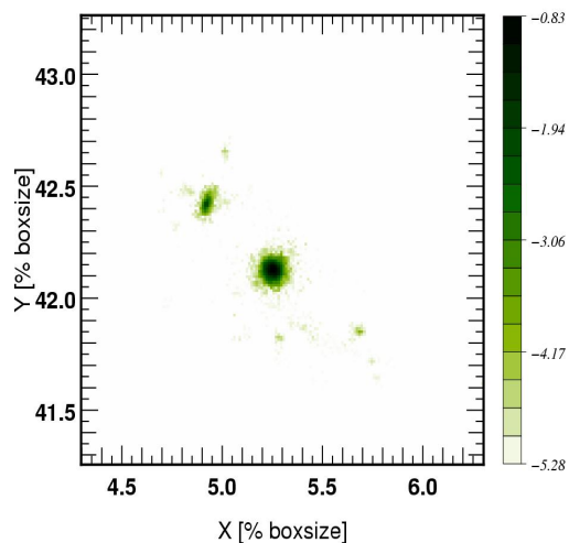
Halo FOF 4 z=5.38: Stellar metal [dex]
