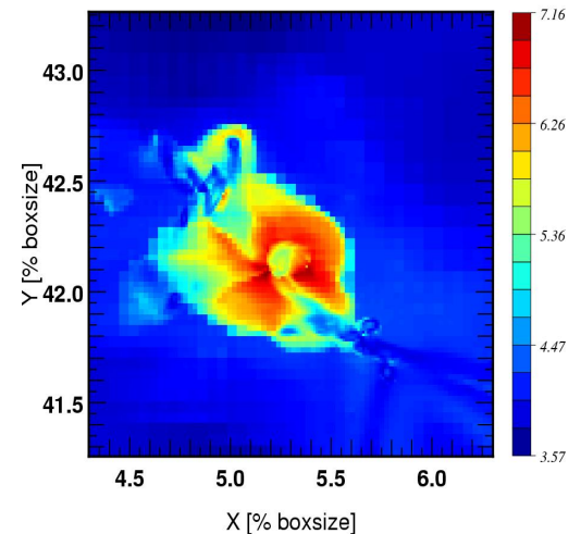
Halo FOF 4 z=5.38 : Velocity V_z [km/s]
