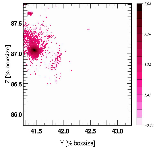
Halo FOF 4 z=4.01: Stellar Mass \rho/\rho_{\text{avg}}
