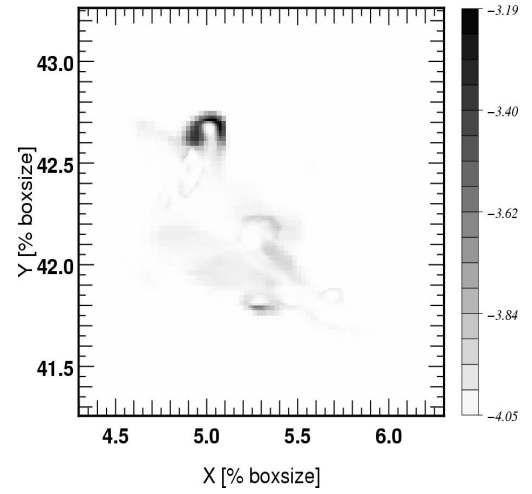
Halo FOF 4 z=5.38: Metallicity [% \rho ]
