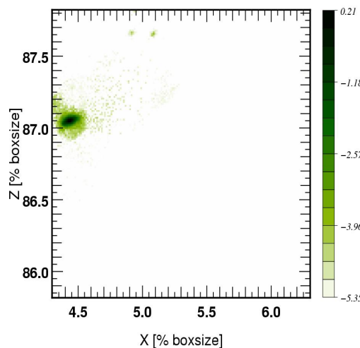
Halo FOF 4 z=4.01: Stellar metal [dex]
