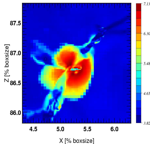
Halo FOF 4 z=5.38 : Velocity V_y [km/s]
