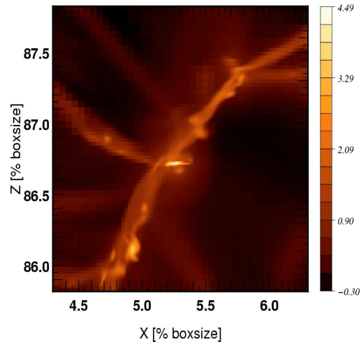
Halo FOF 4 z=5.38: DM Density \rho/\rho_{\text{avg}}
