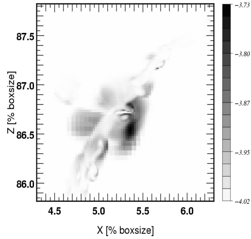
Halo FOF 4 z=5.38: Metallicity [% \rho ]
