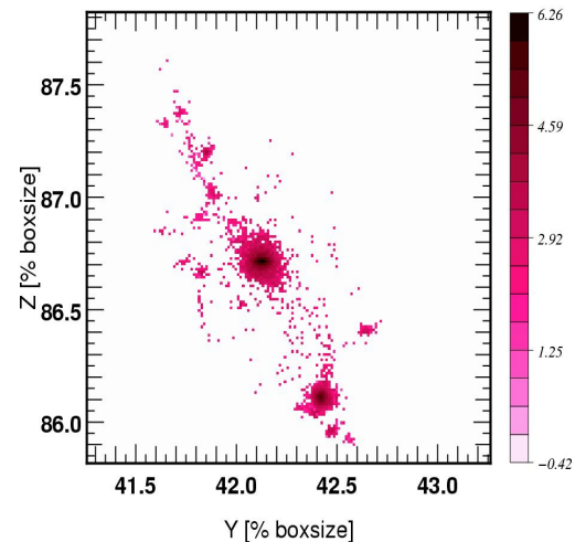
Halo FOF 4 z=5.38: Stellar Mass \rho/\rho_{\text{avg}}
