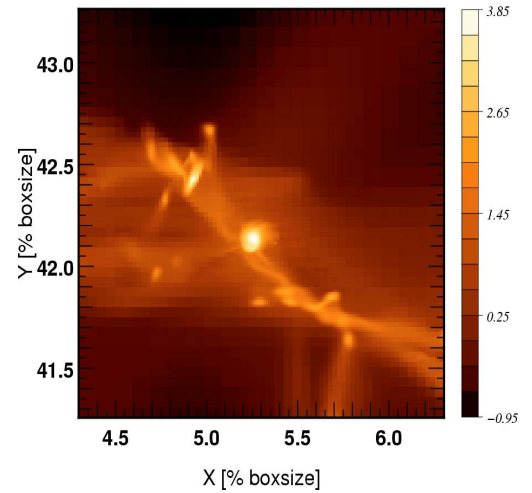
Halo FOF 4 z=5.38: DM Density \rho/\rho_{\text{avg}}
