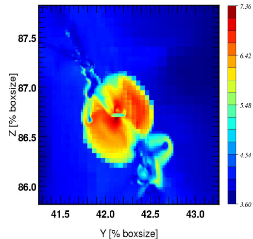
Halo FOF 4 z=5.38 : Velocity V_x [km/s]
