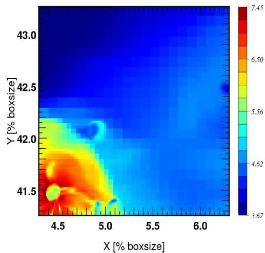
Halo FOF 4 z=4.01: Temperature [K/ \mu ]
