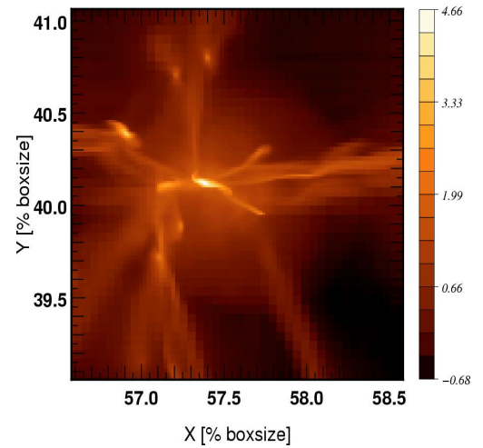
Halo FOF 2 z=4.01: Density \rho/\rho_{\text{avg}}
