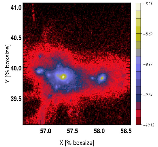
Halo FOF 2 z=5.38: Metallicity [% \rho ]
