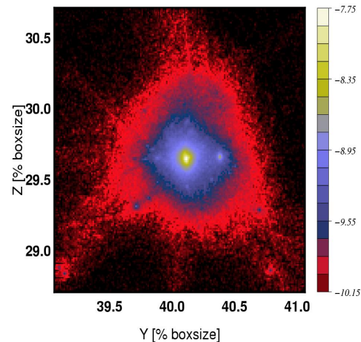
Halo FOF 2 z=4.01: Metallicity [% \rho ]
