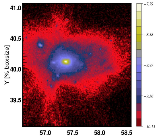
Halo FOF 2 z=4.01: DM Density \rho/\rho_{\text{avg}}
