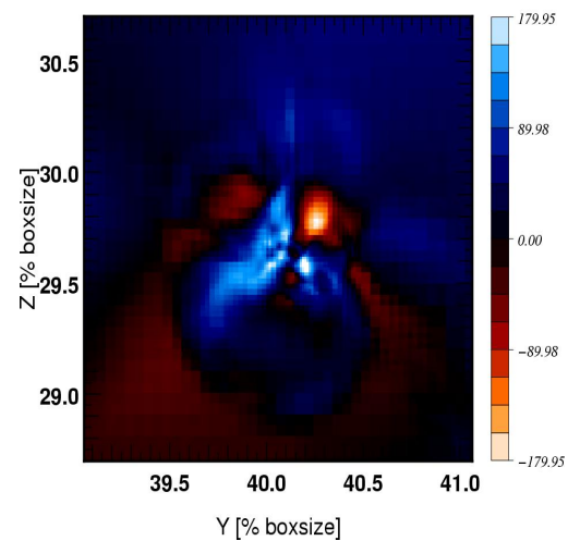
Halo FOF 2 z=4.01: Velocity Vx [km/s]
