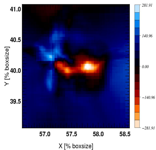
Halo FOF 2 z=4.01: Velocity Vz [km/s]
