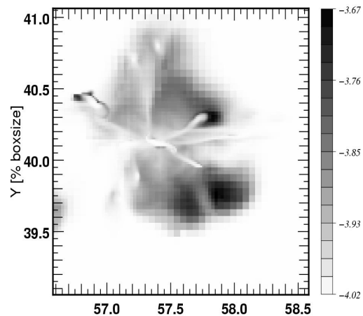
Halo FOF 2 z=4.01: Metallicity [% \rho ]
