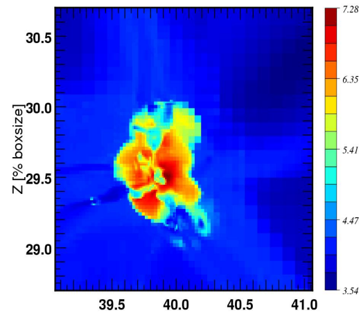
Halo FOF 2 z=5.38: Temperature [K/ \mu ]
