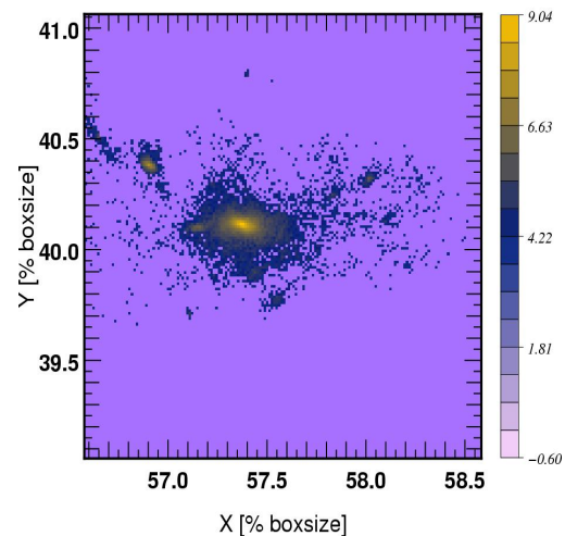
Halo FOF 2 z=4.01: Stellar metal [dex]
