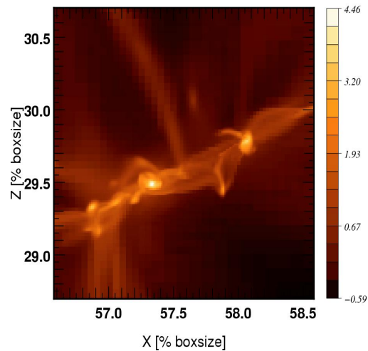
Halo FOF 2 z=5.38: DM Density \rho/\rho_{\text{avg}}
