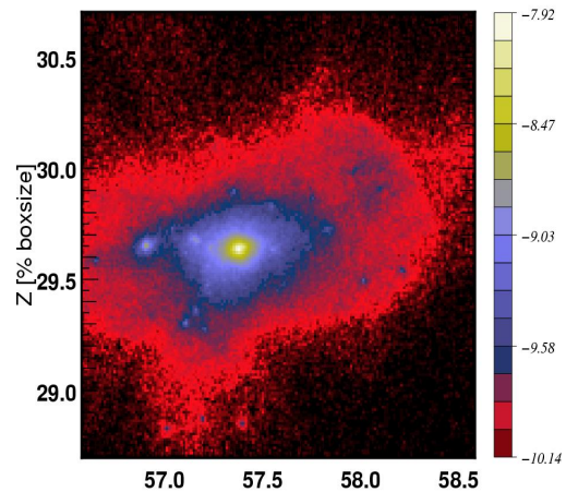
Halo FOF 2 z=4.01: DM Density \rho/\rho_{\text{avg}}
