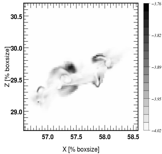
Halo FOF 2 z=5.38: Metallicity [% \rho ]
