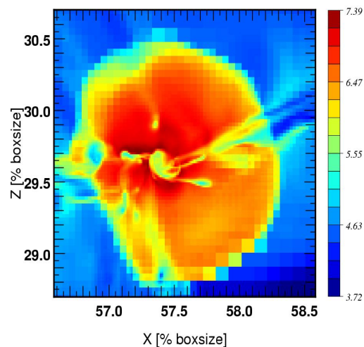
Halo FOF 2 z=4.01: Temperature [K/ \mu ]
