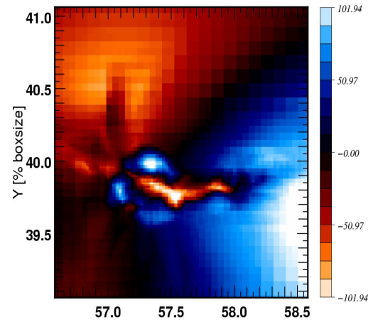
Halo FOF 2 z=5.38: Velocity Vz [km/s]
