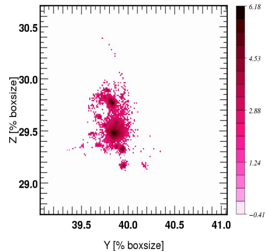
Halo FOF 2 z=5.38: Stellar Mass \rho/\rho_{\text{avg}}
