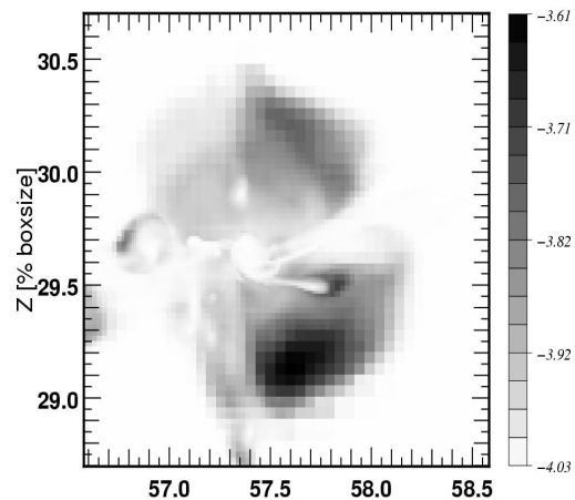
Halo FOF 2 z=4.01: Metallicity [% \rho ]
