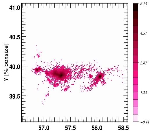
Halo FOF 2 z=5.38: Stellar age [Myear]
