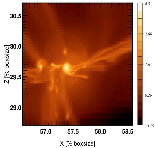
Halo FOF 2 z=4.01: Density \rho/\rho_{\text{avg}}
