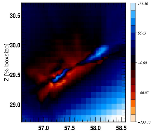
Halo FOF 2 z=5.38: Velocity Vy [km/s]
