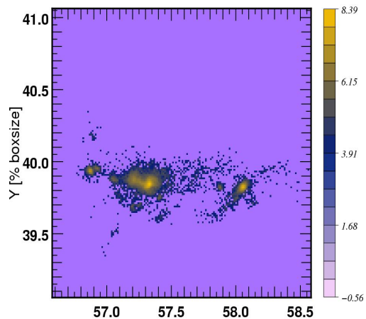
Halo FOF 2 z=5.38: Stellar Mass \rho/\rho_{\text{avg}}
