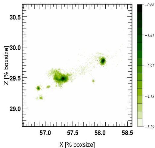
Halo FOF 2 z=5.38: Stellar metal [dex]
