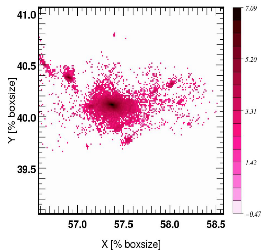
Halo FOF 2 z=4.01: Stellar age [Myr]
