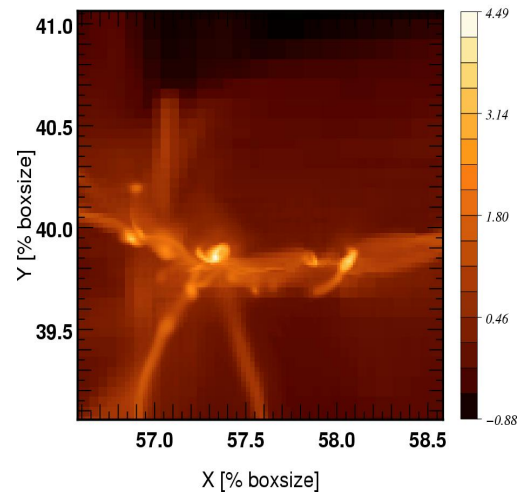
Halo FOF 2 z=5.38: DM Density \rho/\rho_{\text{avg}}
