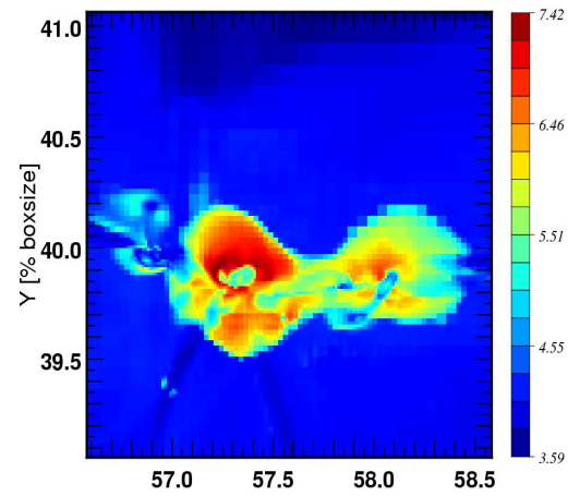
Halo FOF 2 z=5.38: Temperature [K/ \mu ]
