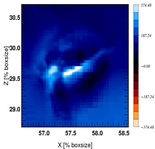
Halo FOF 2 z=4.01: Velocity Vy [km/s]
